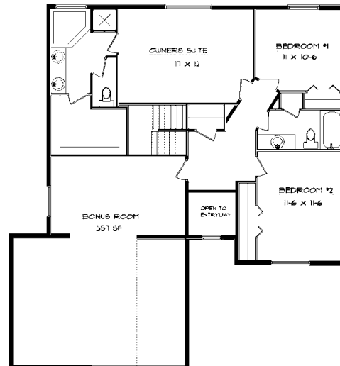
Upper Floor
